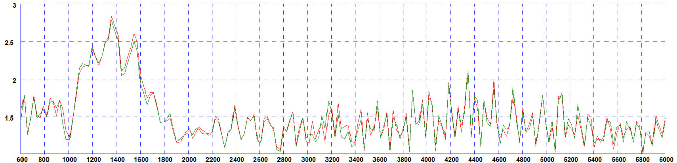
Typical VSWR*
